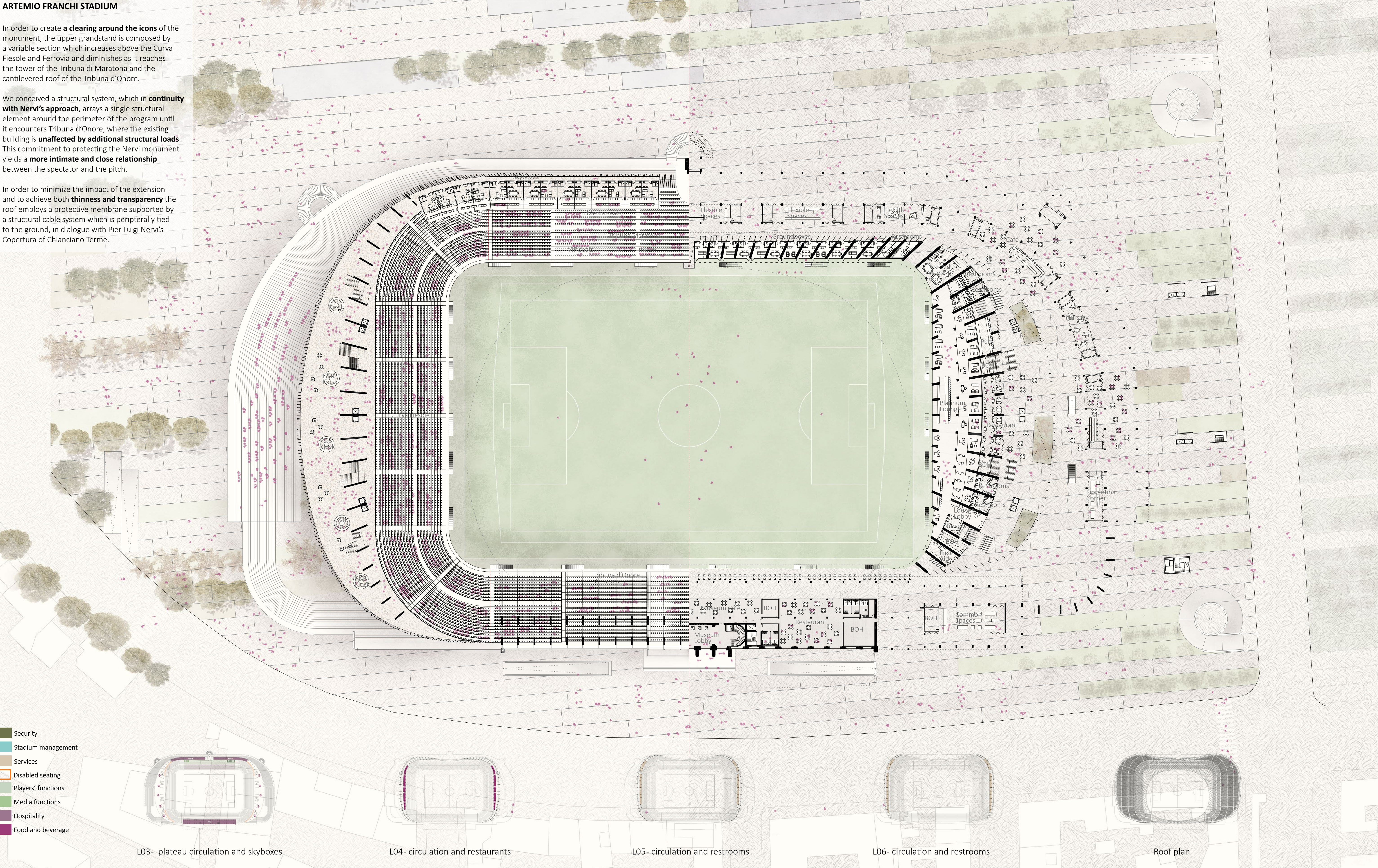
CONTINUITA' | Il Franchi Ground Floor | Level 03 | Plan 1:500
